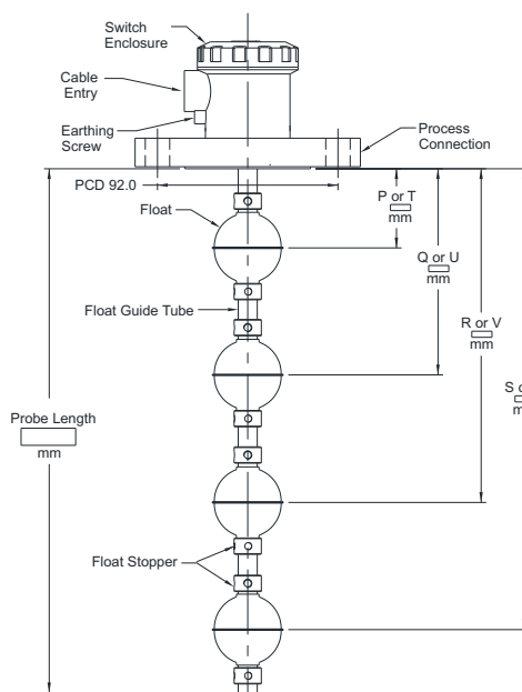
Flange Connection
