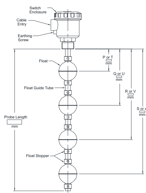
Threaded Connection
