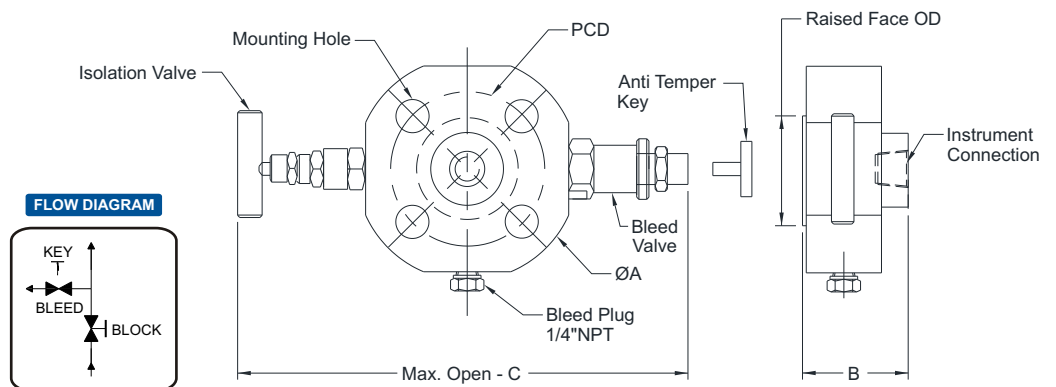
Monoflange Single Block & Bleed Valve
