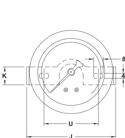
Type R3 (Bayonet ring)
