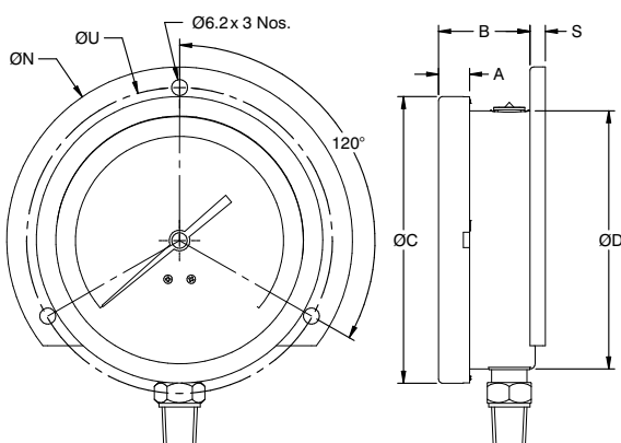
Type B1, (Bayonet ring)
