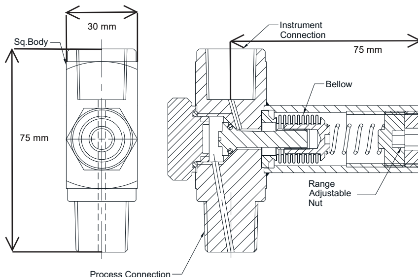
Pattern 1, 2, 3 (Bellow type)
